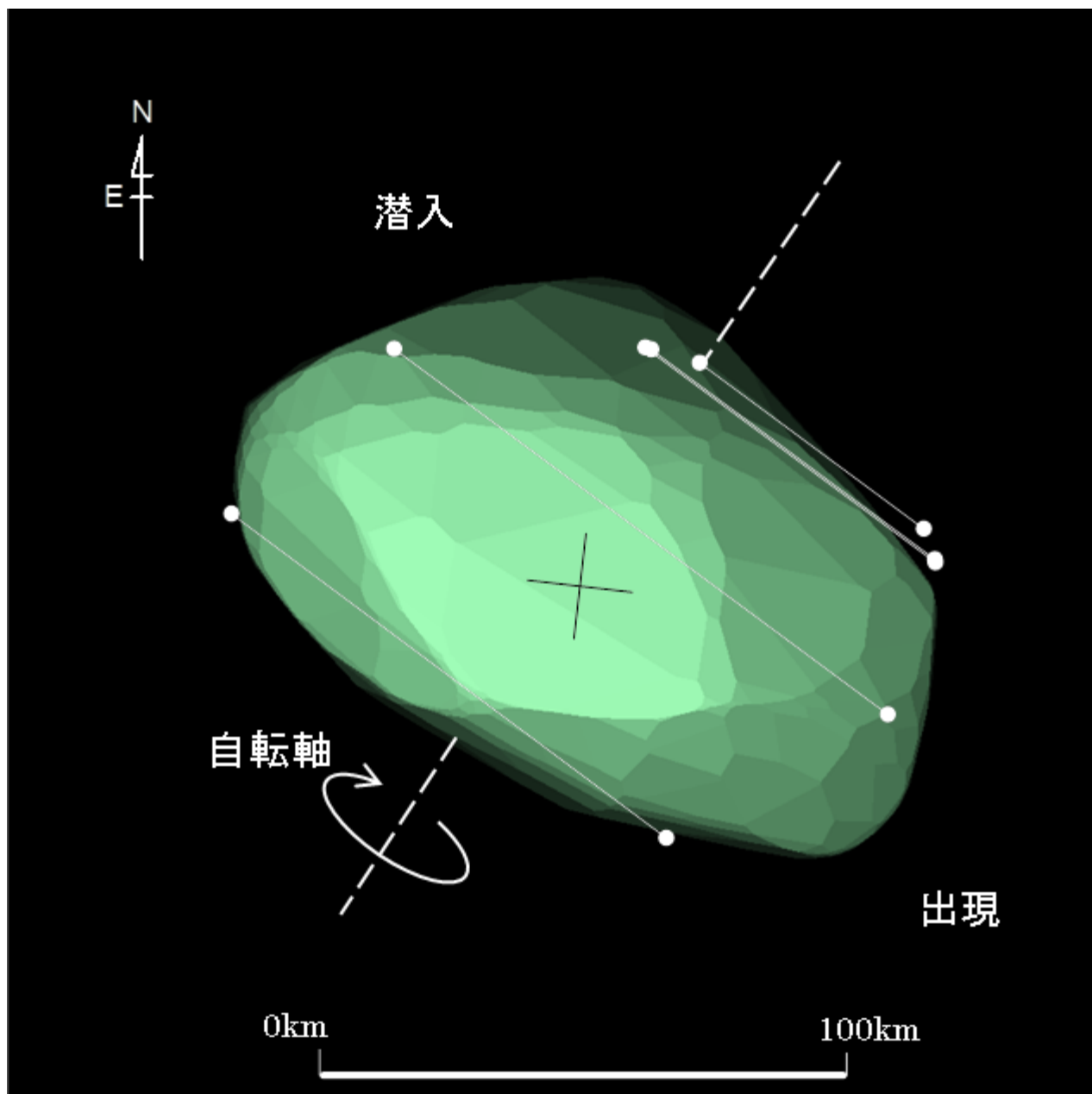
(127)Johanna 2014年9月8日 20h09m12s UT DAMIT Model 444 ( \lambda = 98 , \beta = -60 ) P = 146.5^\circ , \beta_e = -21.4^\circ , \lambda_e = -211.8^\circ , Scale Factor 1:93.2, k = 0.969 , B = 76.5^\circ
